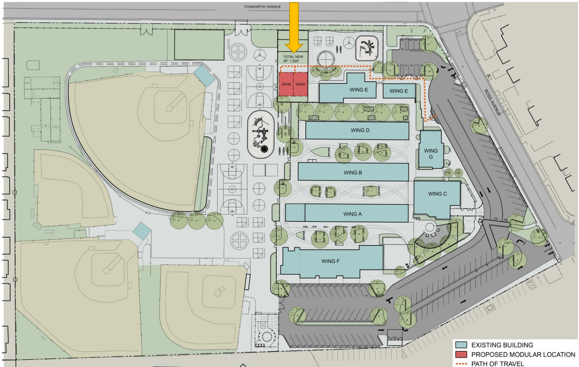
STEINDORF EXTENDED CARE NEW MODULAR CLASSROOMS - OPTION 1 CAMBRIAN SCHOOL DISTRICT
